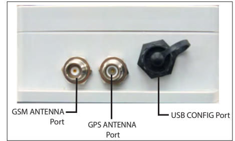
Enclosure Top View
